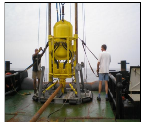
Vibrocore unit
